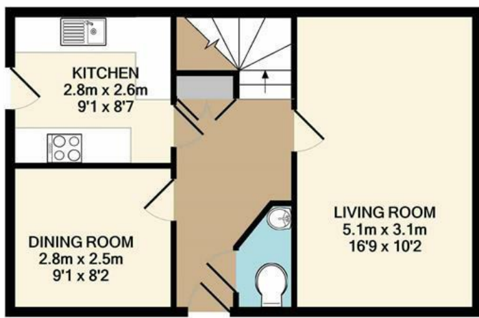
GROUND FLOOR APPROX. FLOOR AREA 40.6 SQ.M. (437 SQ.FT.)
